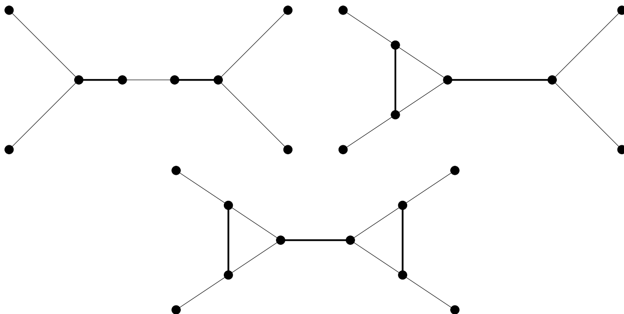
Figure 2. Three cases of transversal intersection.
