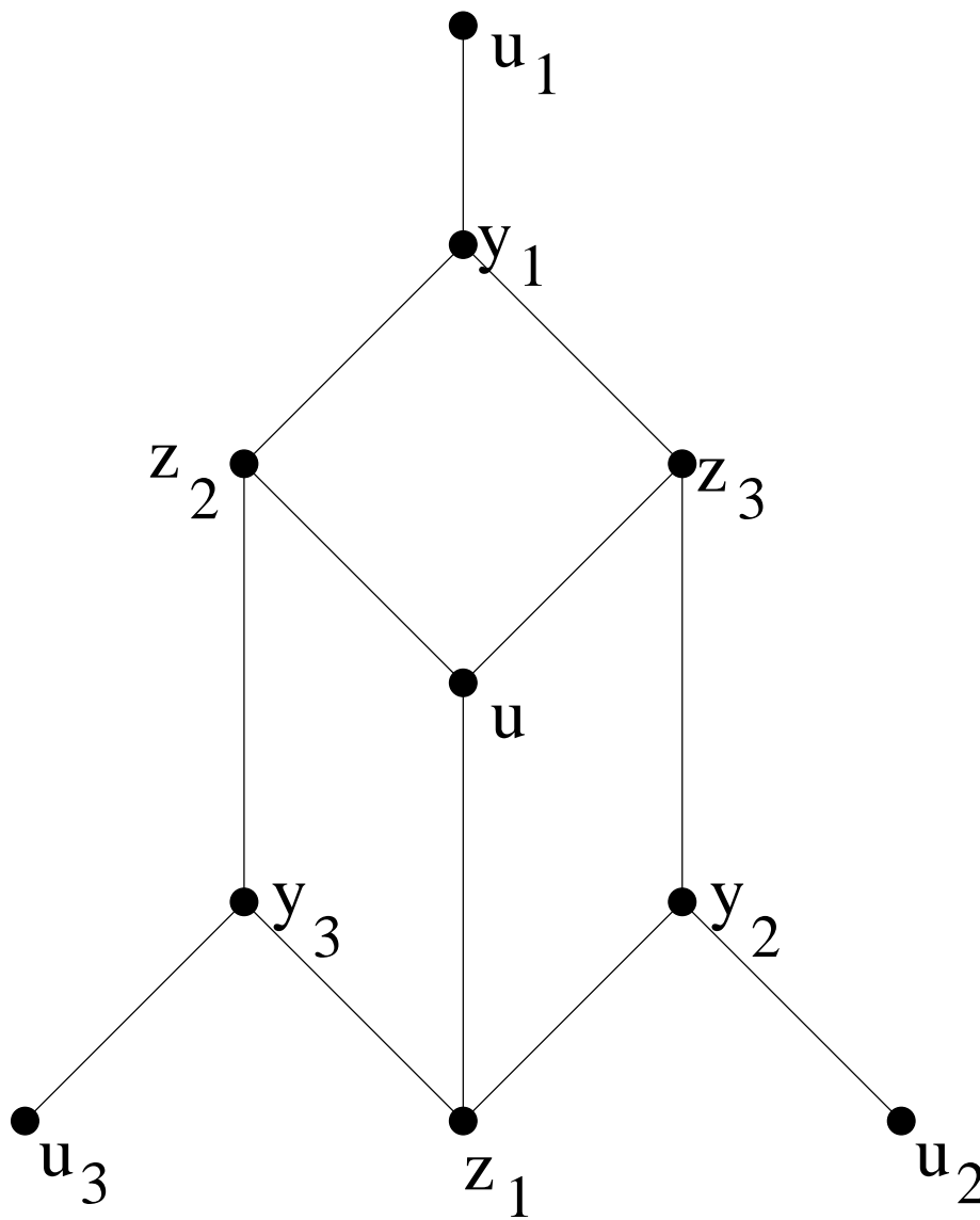
Figure 8. A cube extension.
