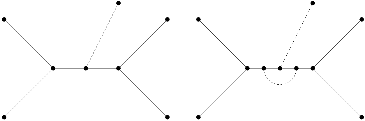
Figure 4. Augmentations of type A.
