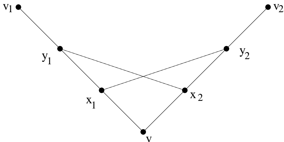
Figure 7. A cross extension.
