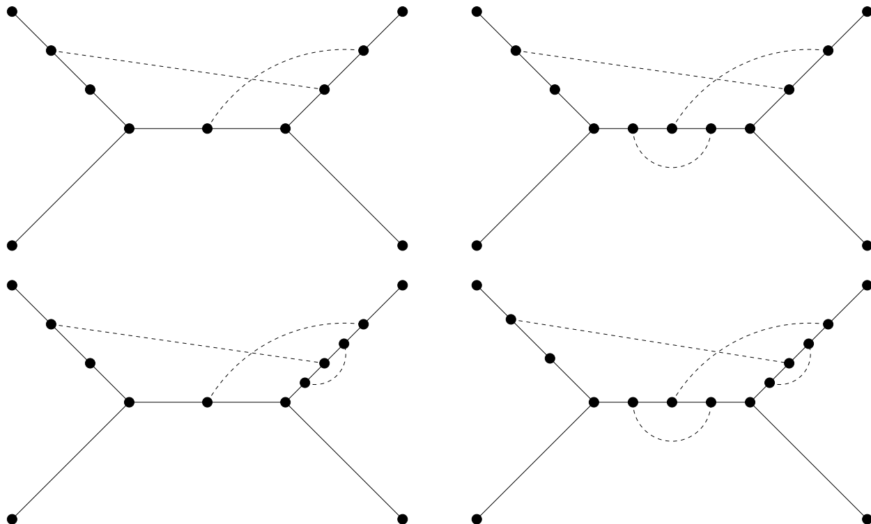
Figure 6. Augmentations of type C.
