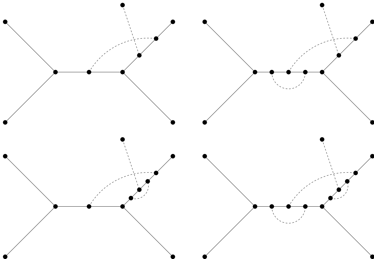
Figure 5. Augmentations of type B.
