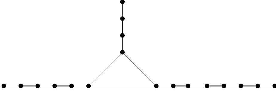
Figure 1. An octopus \Omega and an \Omega -compatible matching.
