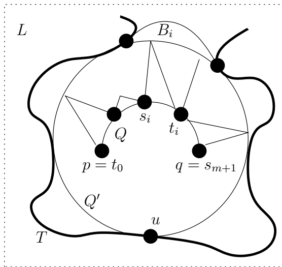
Figure 2: Illustration of Lemma (2.5)
