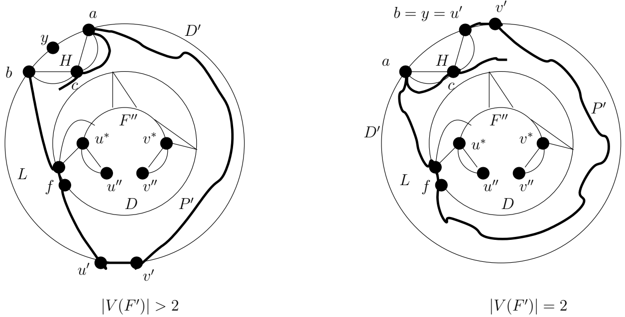
Figure 5: Subcase 2.1
